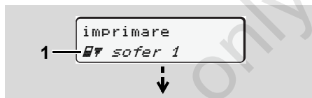
1. Meniu principal
